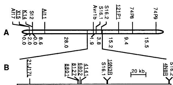
Fig. 2. Genetic and physical maps of the linkage group analyzed. (A) Genetic map. The map was constructed by analysis of 100 F_2 progeny from a cross of P6497 \times P7064 using MAPMAKER 1.0. All molecular markers are RAPD markers except 121P1, 74P8, and 74P9, which are restriction fragment length polymorphisms. Codominant alleles of the underlined markers were used for this study. Avr1b is a phenotypic marker. Distances are in centimorgans. (B) Physical locations of markers on a 200-kb bacterial artificial chromosome contig spanning Avr1b . Underlined markers were used in this study. Marker 8127 lies within Avr1b . The expansion lines show the position and orientation of the contig on the genetic map.
